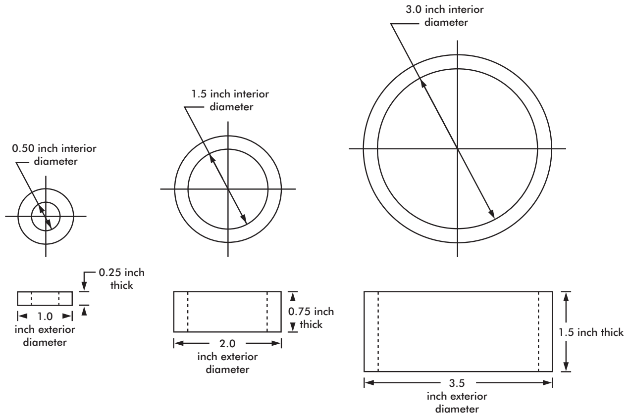
Figure B1. Projection test gauges
