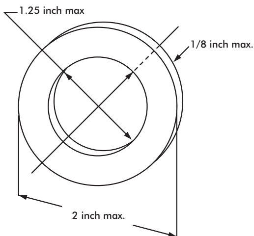
Figure B2. Projection test gauge for suspended swing assemblies and slides
